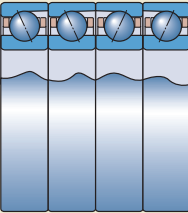
Tandem face-to-face arrangement Designation suffix QFC
