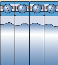
Face-to-face and tandem arrangement Designation suffix QFT
