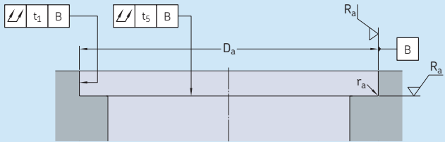
Geometrical accuracy for bearing housing seats
