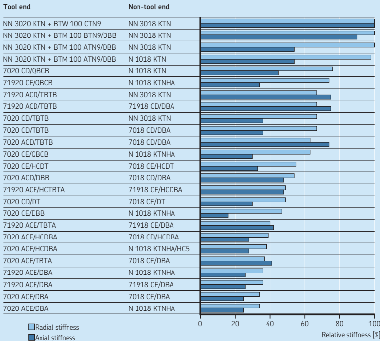
Relative stiffness of typical spindle bearing systems
